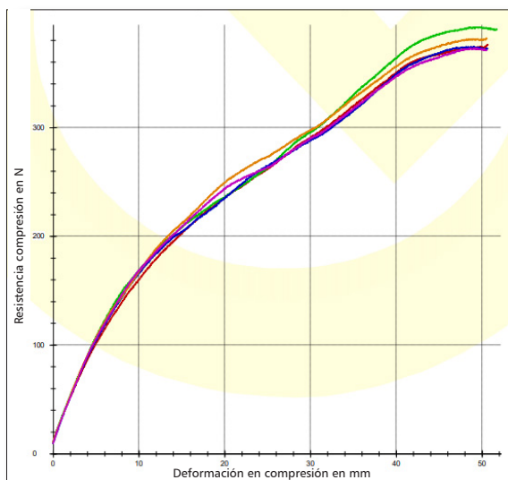
Strength/deformation obtained during the compression test of a Type 200 bucket
